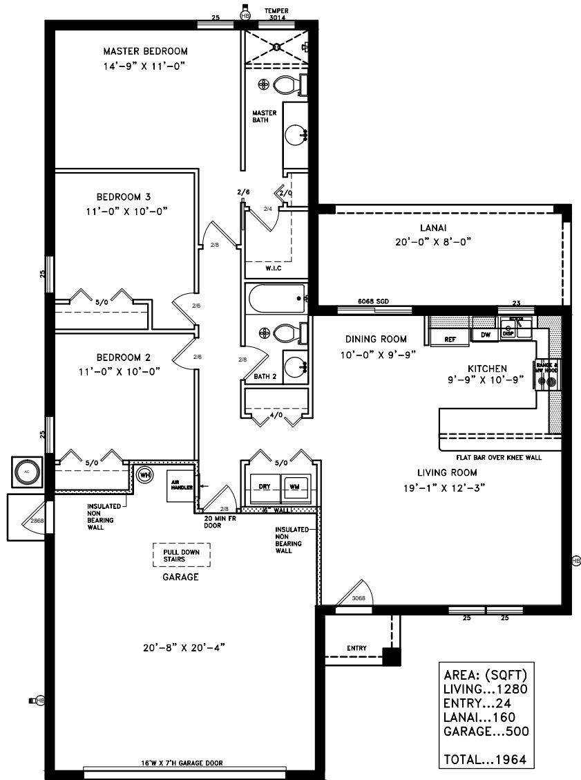
THE ARCADIA (41'-6"W X 59'-10"D)
